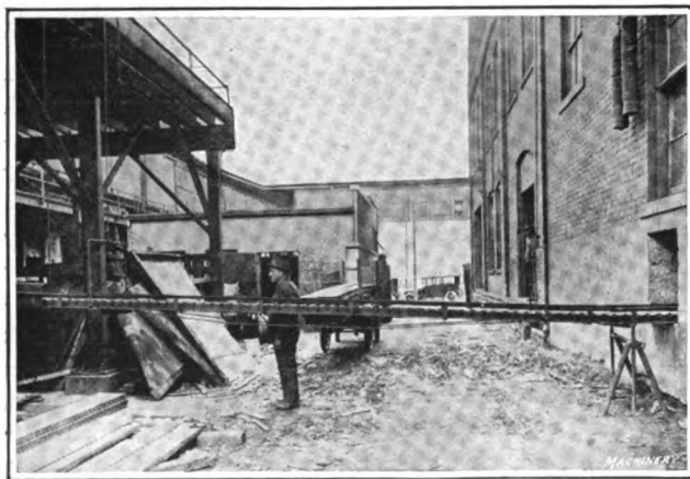
Fig. 37—This illustration shows the gravity carrier leading from the spiral chute shown in Fig. 36 to the machining shop. The carrier is suspended on cables so that it may be raised to provide the necessary head room for a team to go underneath
